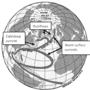
The Atlantic Meridional Overturning Circulation, after Rahmstorf, Nature 1997
